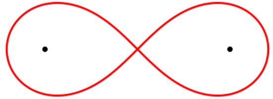
The lemniscate of Bernoulli and its two foci
